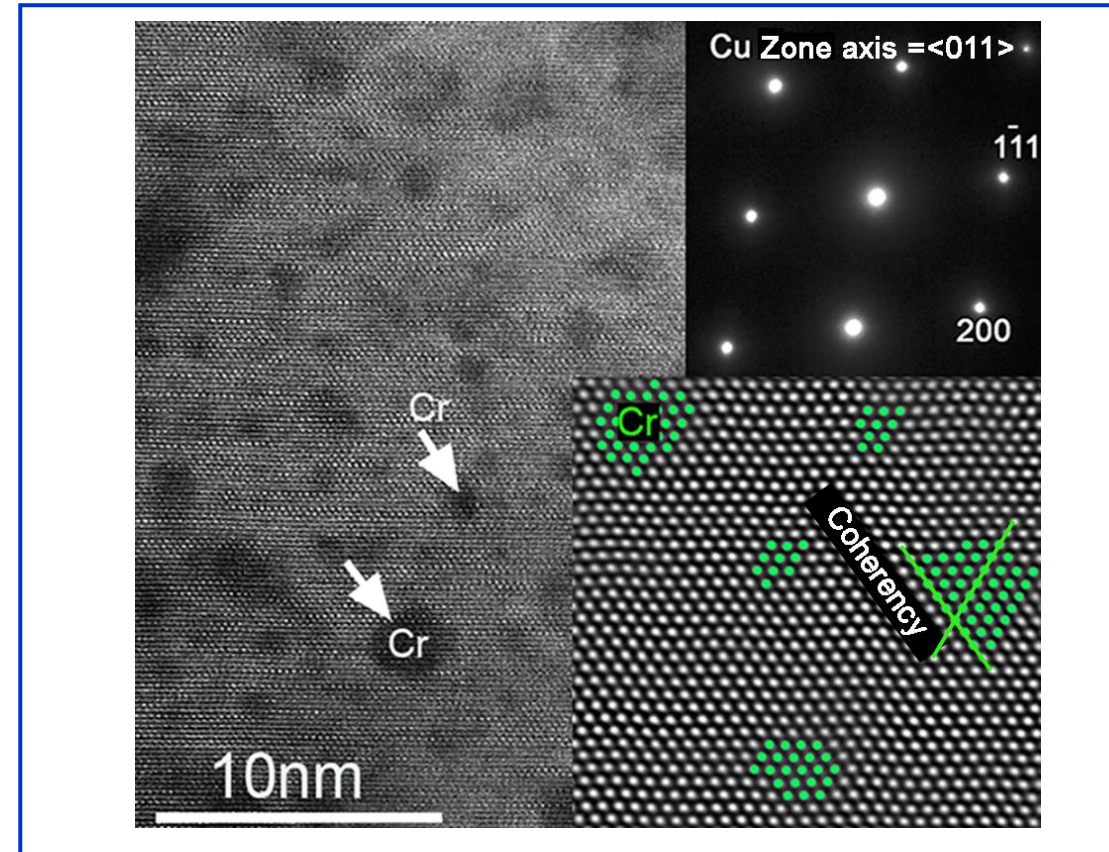
Figure: An atomic-resolution, high-angle annular dark-field image of an aged sample showing uniformly distributed Cr precipitates (dark contrast in main image). A fast Fourier transformed image (lower inset) shows coherent interfaces (such as the one indicated by a green line) between the Cu matrix and the precipitates (shown in green). Due to the coherent structure between the precipitates and the matrix, only one set of diffraction spots appears in the selected area diffraction pattern (top inset).
