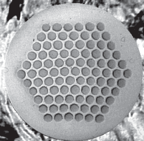
Cross-Section of a Cu-(Nb-47Ti-Nb) Composite Wire
