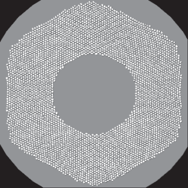
Multifilamentary Cu/Nb-47Ti Composite SSC Type Wire in Transverse Cross-section
