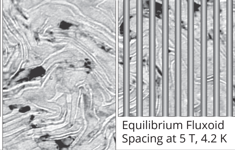
Multifilamentary Cu/Nb-47Ti Composite SSC Type Wire in Transverse Cross-section
