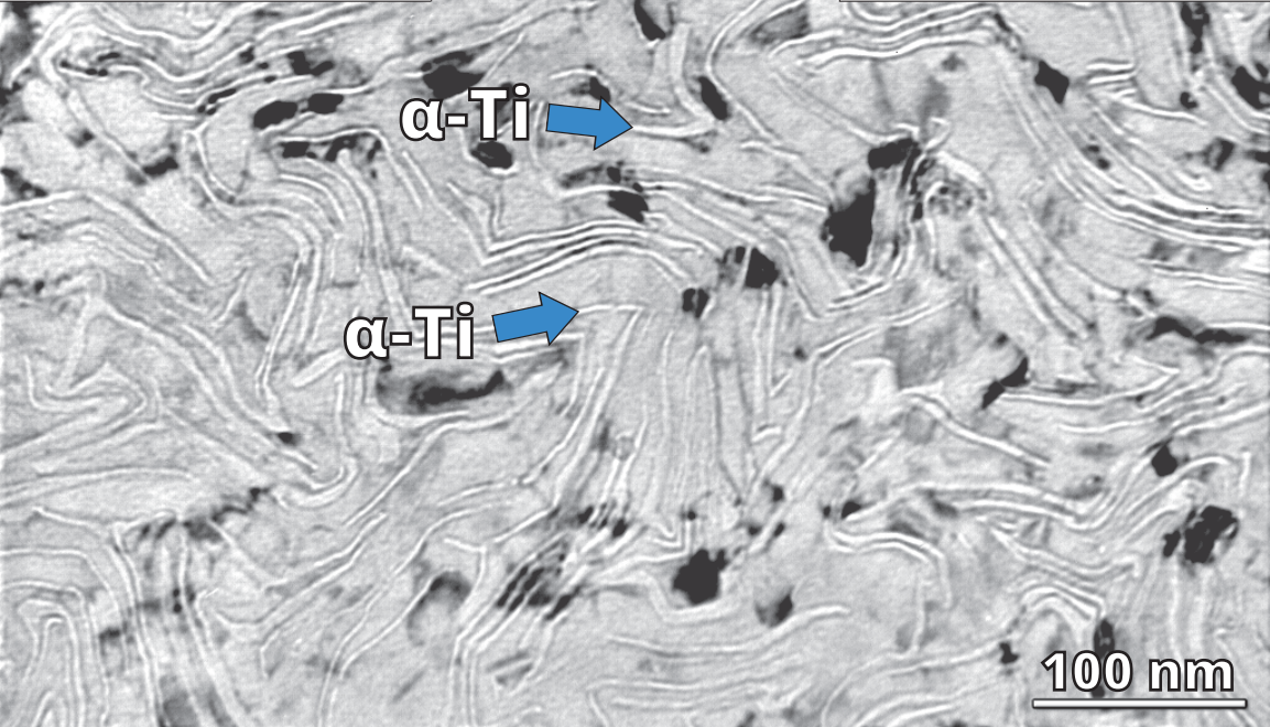
Multifilamentary Cu/Nb-47Ti Composite SSC Type Wire in Transverse Cross-section
